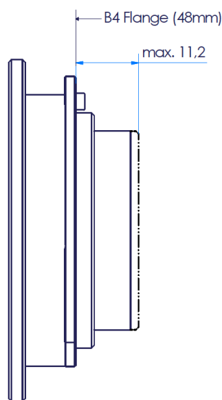
III. 1: max. measurements of input lens
